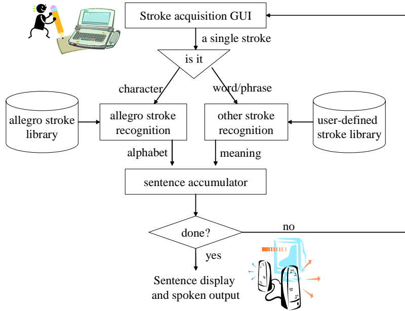
Figure 3. Procedure of the shorthand recognition system.
